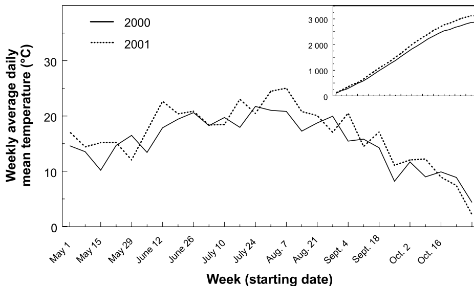
FIGURE 2. Weekly average daily mean temperature in Ottawa, Ontario, for 2000 and 2001, from 1 May to 31 October. Inset: cumulative daily mean temperature.
