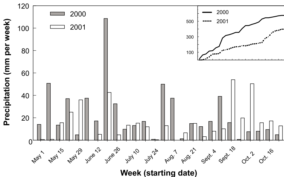
FIGURE 1. Weekly precipitation in Ottawa, Ontario, for 2000 and 2001, from 1 May to 31 October. Inset: cumulative precipitation.
